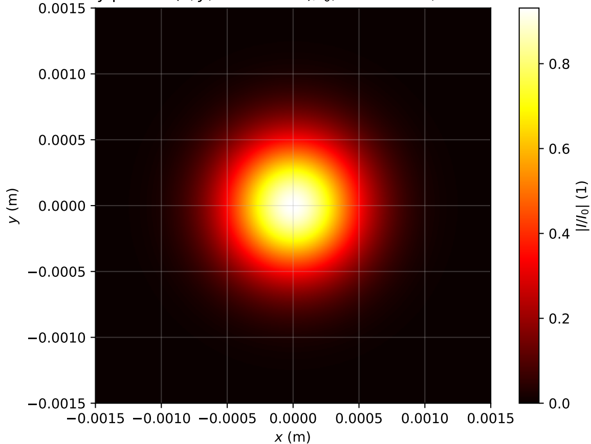
Intensity profile I(x, y, z = 0.796m)/I_0 , Pin=0.2Pcr, artificial time
